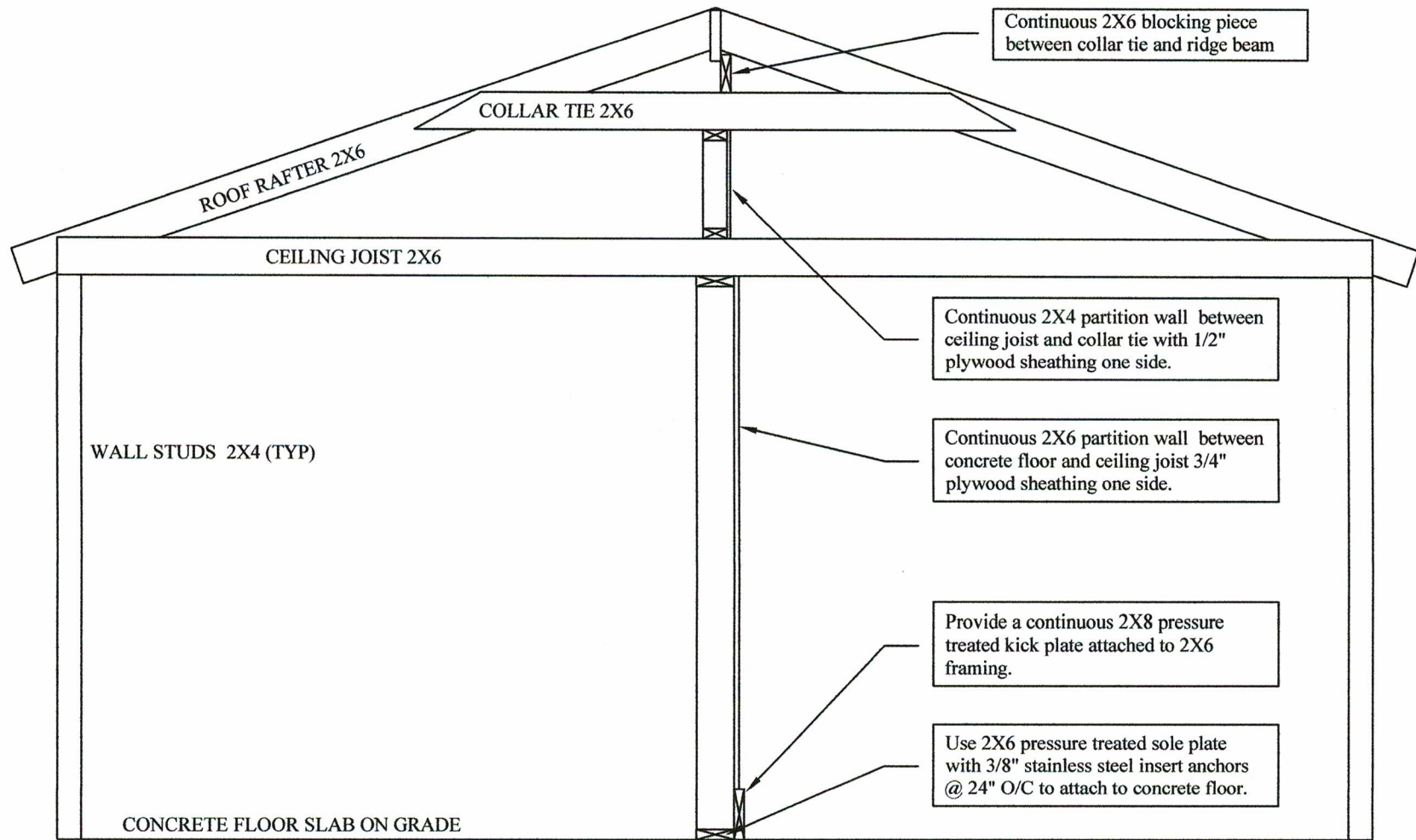
Proposed Framing Details Section View @ West Elevation Scale 1/2"=1'
