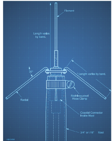
The diagram of our simple ground-plane antenna, using PVC pipe as a support mast.
